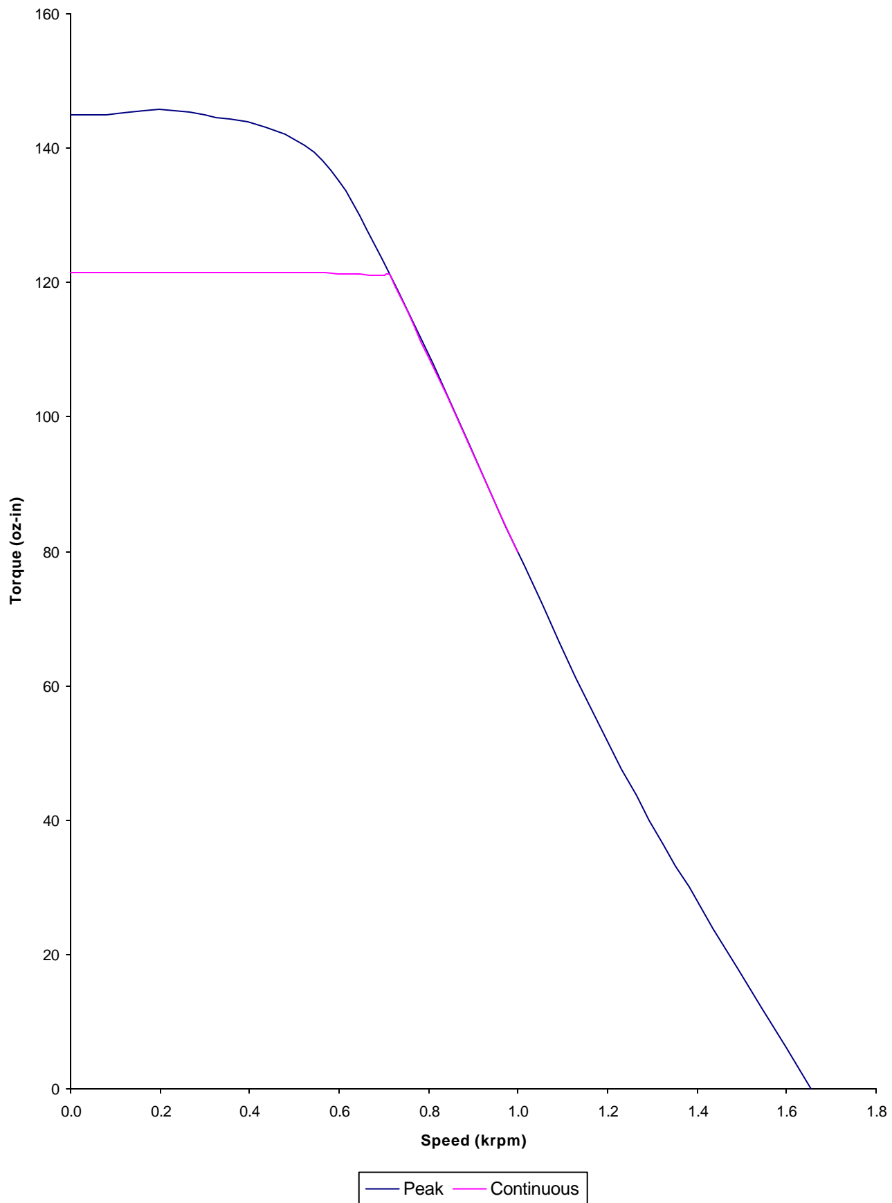
SM3416D Torque vs. Speed at 24 VDC using a PS24V8A supply
